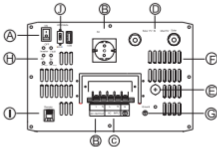
Figure 3.1: Rear Panel
